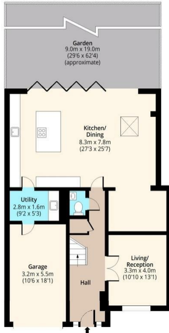
Ground Floor Approx. 106.65 Sq. meters (1148 Sq. feet)
